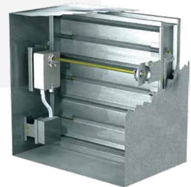
MFSD with actuator mounted inside
